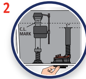
Set Adjustable Overflow Tube.
